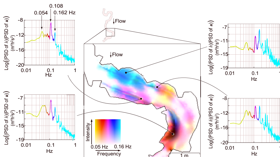
Fig. 5. Frequency and intensity contour of product of power spectral density (PSD) of h and PSD of u obtained by numerical simulation. Color, used in contour, is subtractive color mixture processes of colors, whose hue corresponds to frequency as shown in line plots, and color saturation corresponds to intensity of spectrum at each point.
