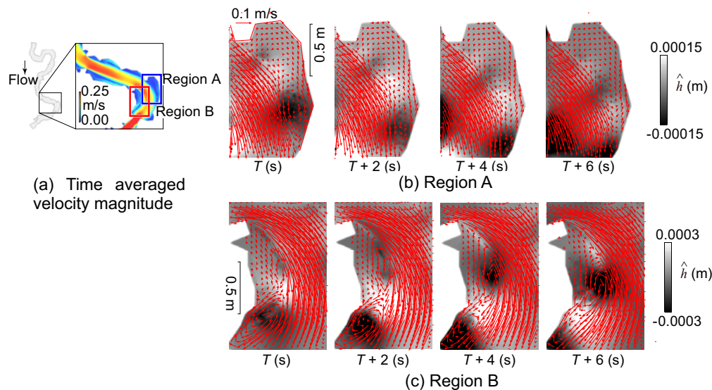
Fig. 4. Snapshot of the contours of fluctuation components. Regions A and B correspond with the regions shown in Fig. 2. Back ground contours indicate fluctuation of water depth. Dents of water surface, shown as dark shade in contour, correspond to centers of vortices. Behavior of vortices in calculated result corresponds well to observed result shown in Figs. 3(b) and 3(c).
